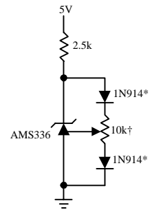
2.5V Reference with Minimum Temperature Coefficient
